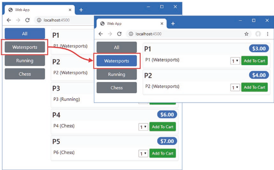
Figure 15-8. Displaying products
