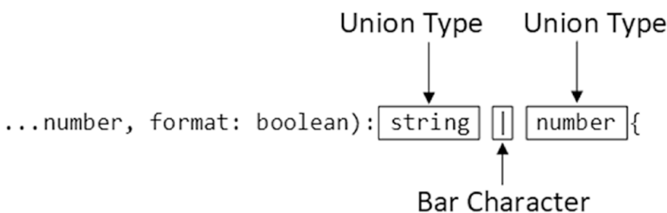
Figure 7-2. Defining a type union
