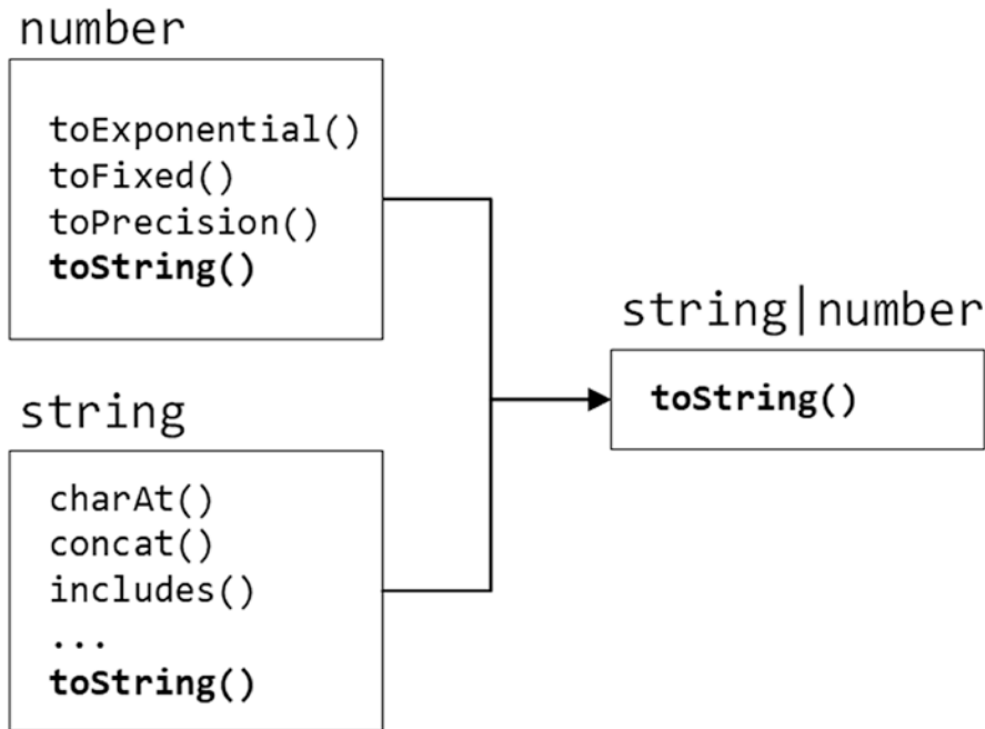
Figure 7-3. The effect of a type union
