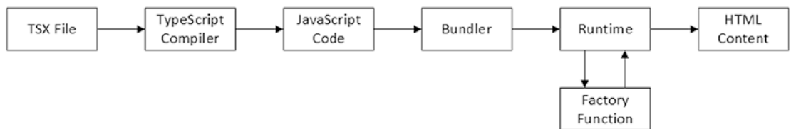
Figure 15-6. Transforming JSX
