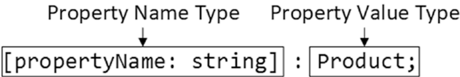
Figure 11-10. An index signature
