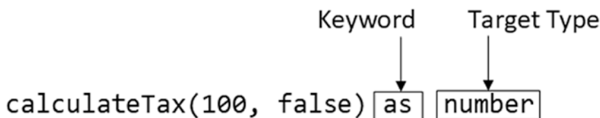
Figure 7-4. Asserting a type
